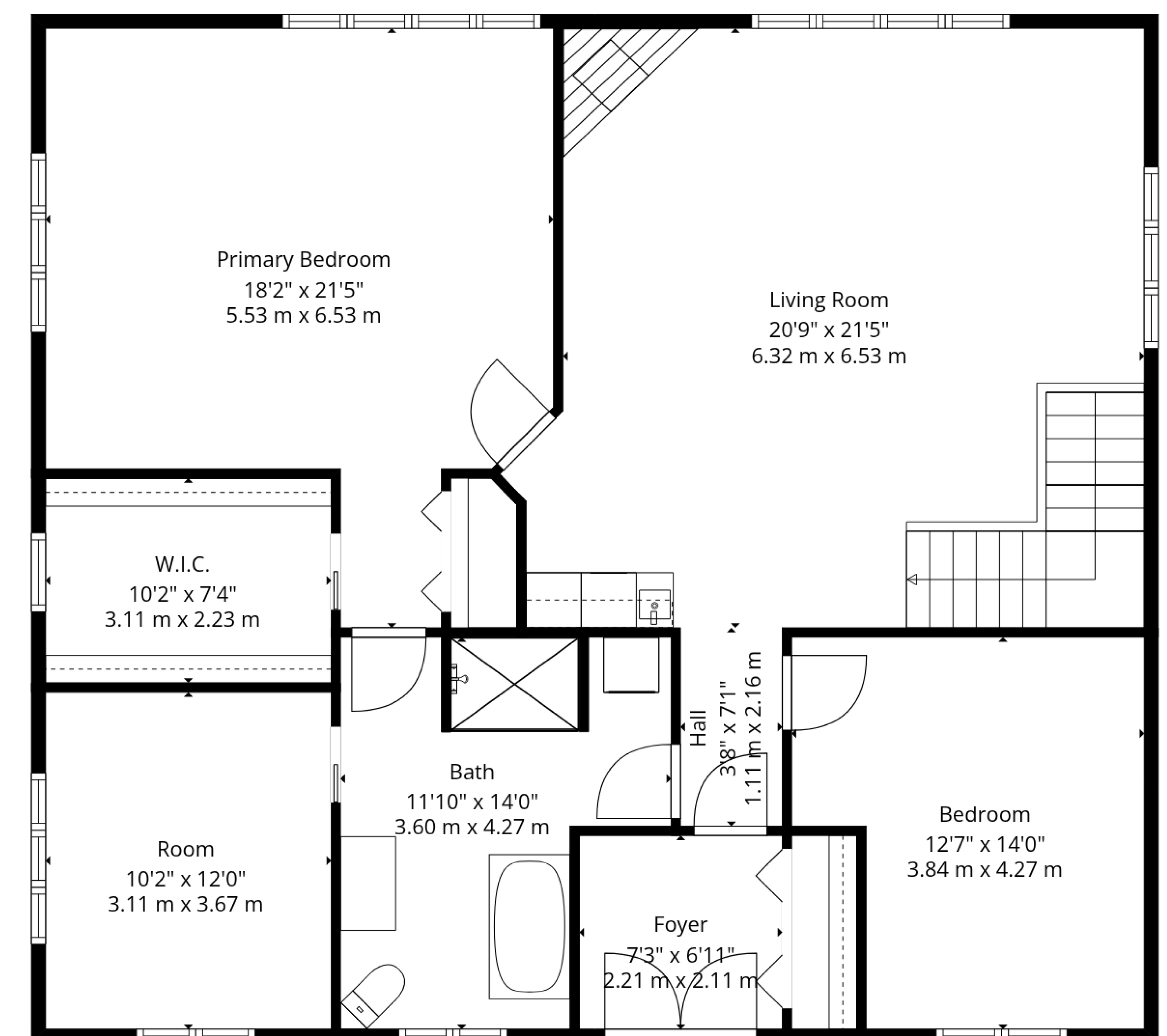
Main Floor
