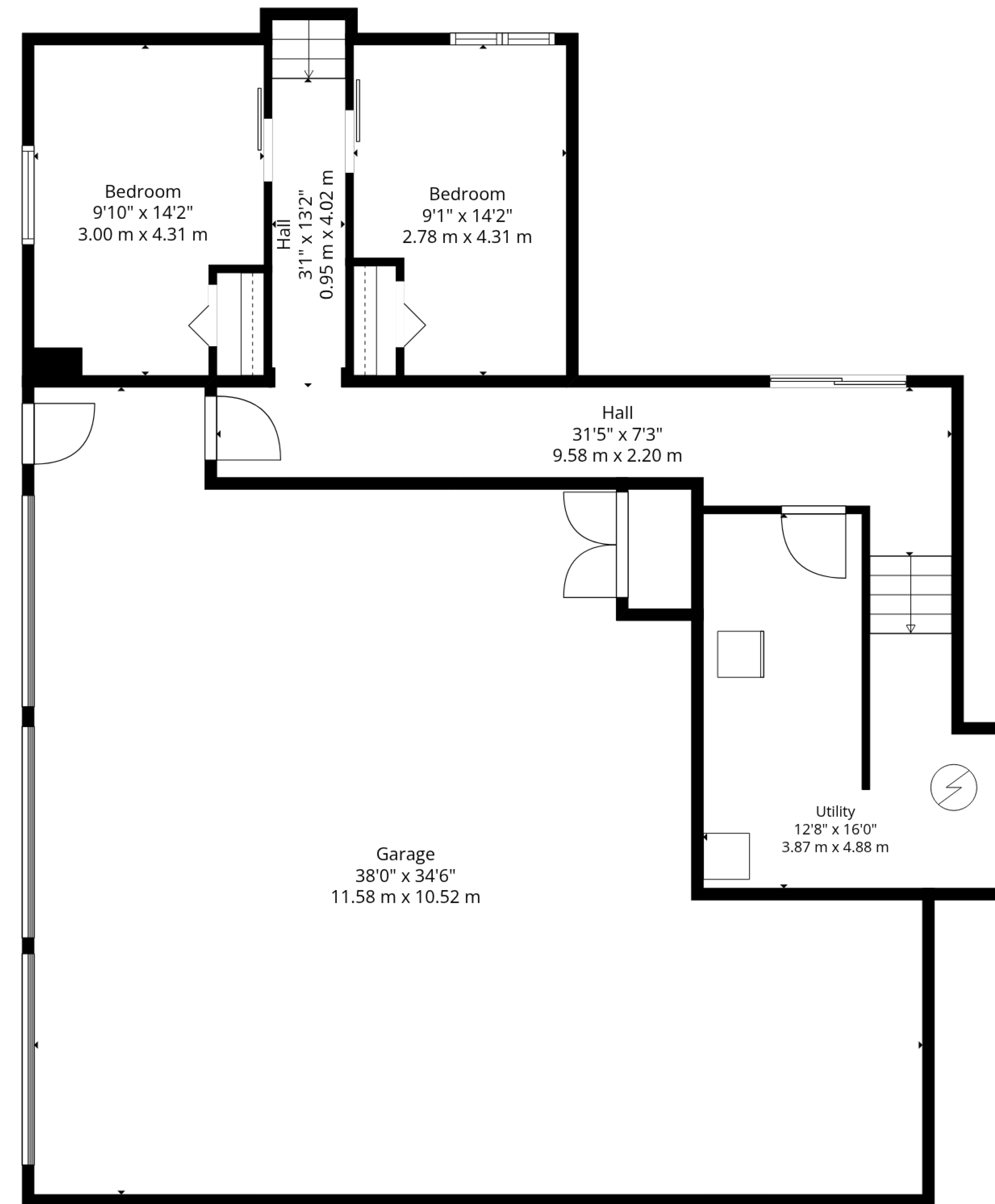
Lower Level
